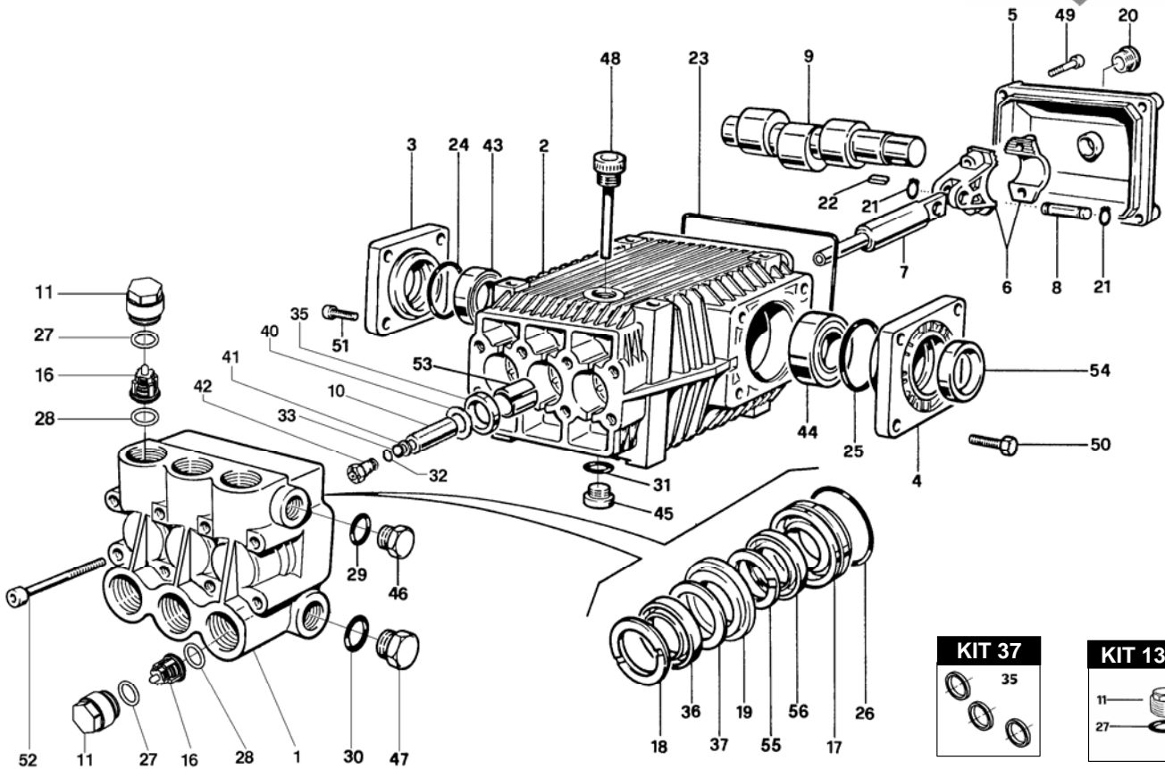
KIT 90
